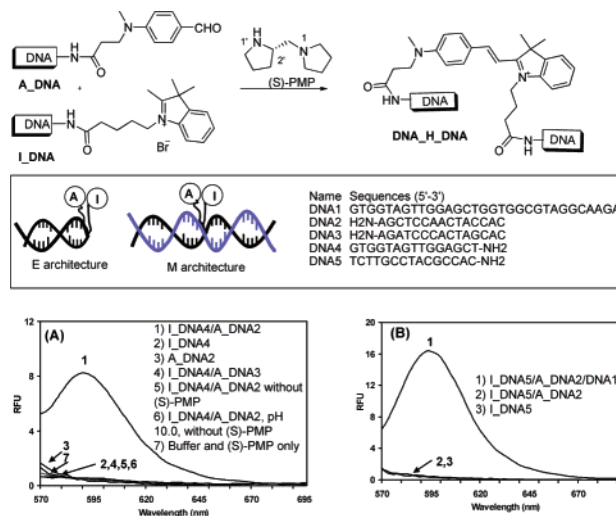
Figure 1. Relative fluorescent intensity of hemicyanine DPC reaction mixtures. DPC reactions were performed using 0.2 \mu\text{M} reagent strands (and equimolar template for M architecture) at RT for 140 min in 10 mM ( S )-PMP, 50 mM sodium phosphate (NaPi), 1 M NaCl, pH 8.4 unless otherwise specified. Results for E and M architecture are shown in (A) and (B), respectively.
